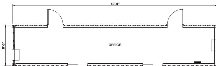
40' x 8' CONTAINER OFFICE
