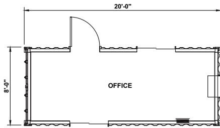
20' x 8' CONTAINER OFFICE
