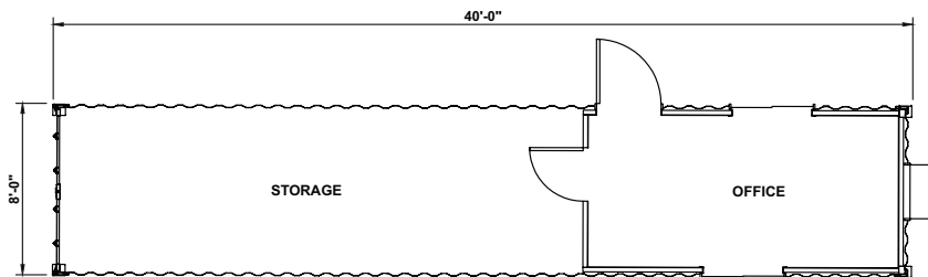
40' x 8' CONTAINER OFFICE & STORAGE COMBO
